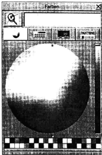
Abb.4: ColorPanel
